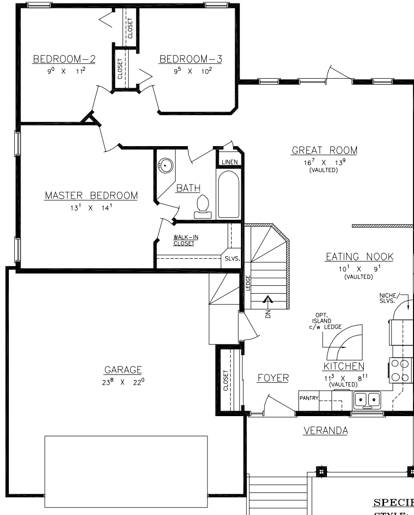
FLOOR PLAN
